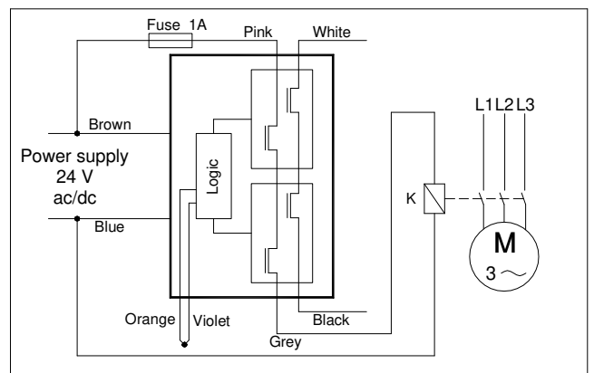
Fig. 3 Connections example for cat.1
