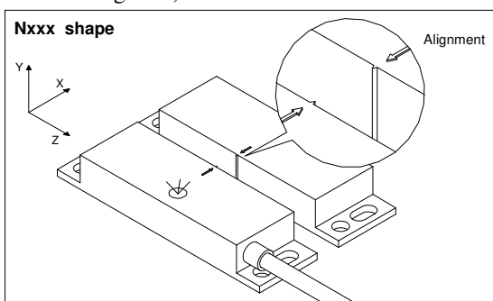
Fig. 1 Sensor alignment
