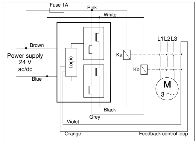
Fig. 2 Connections example for cat.3
